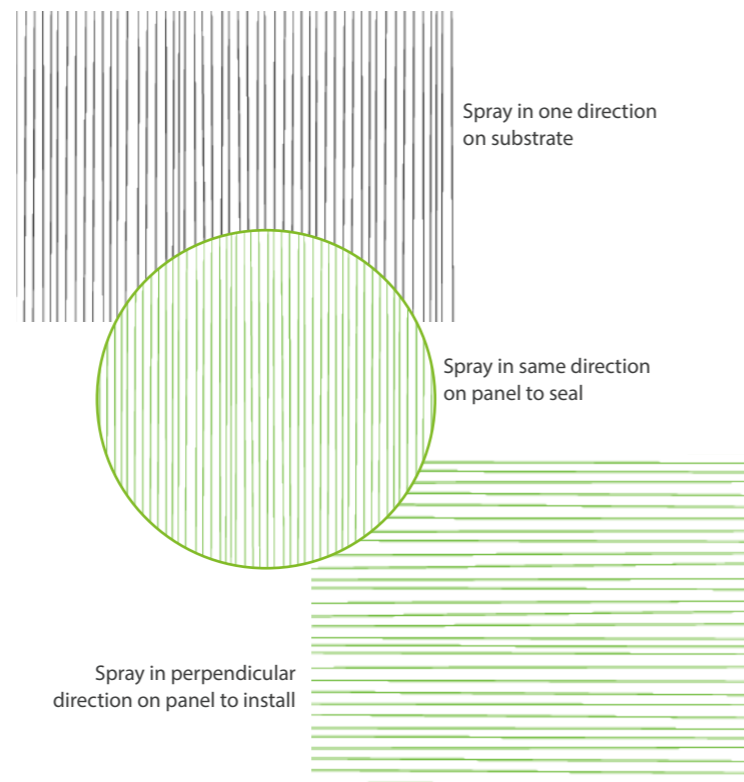
Figure 1. Substrate & Panel Spray Patterns
